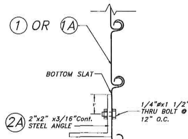
SECTION X2
