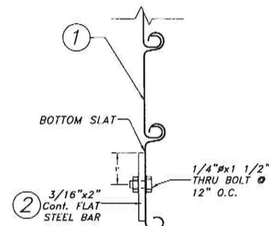
SECTION X1
