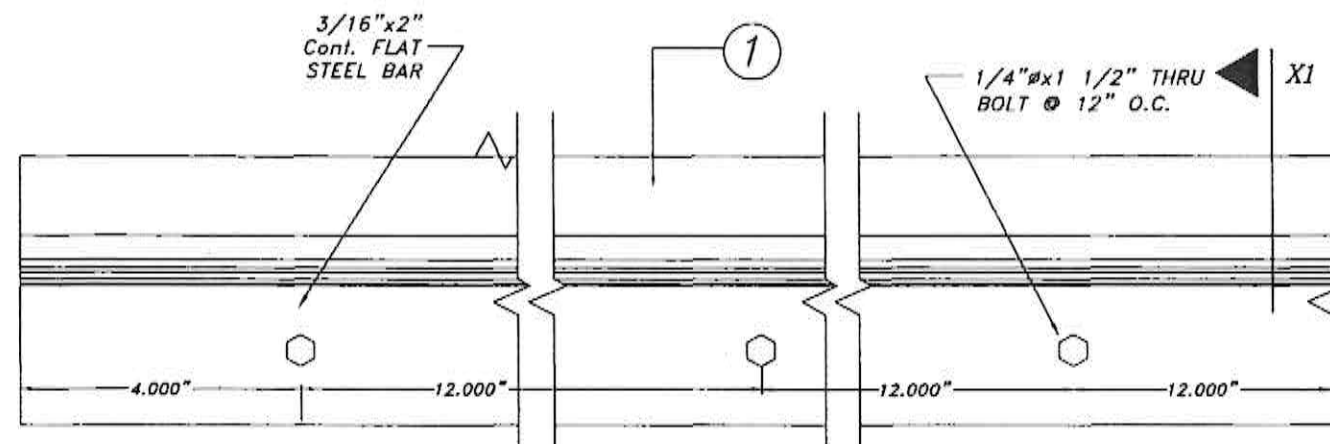
ELEVATION ② BOTTOM BAR REQ'D. ONLY FOR SLAT ① SCALE : 3/8" = 1"
