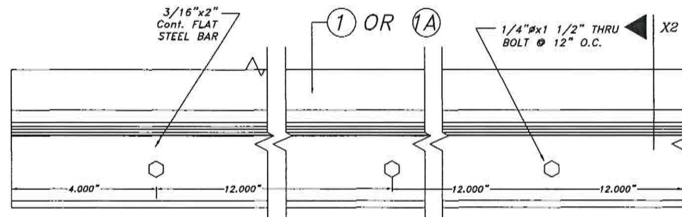
ELEVATION ②A BOTTOM BAR REQ'D. FOR SLATS ① OR ①A SCALE : 3/8" = 1"
