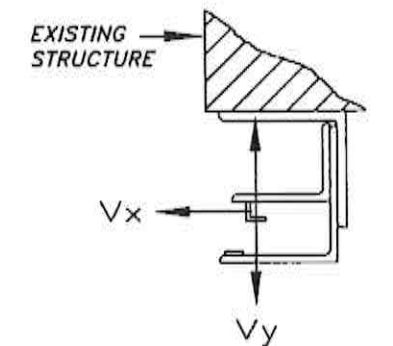
LOAD DIAGRAM
