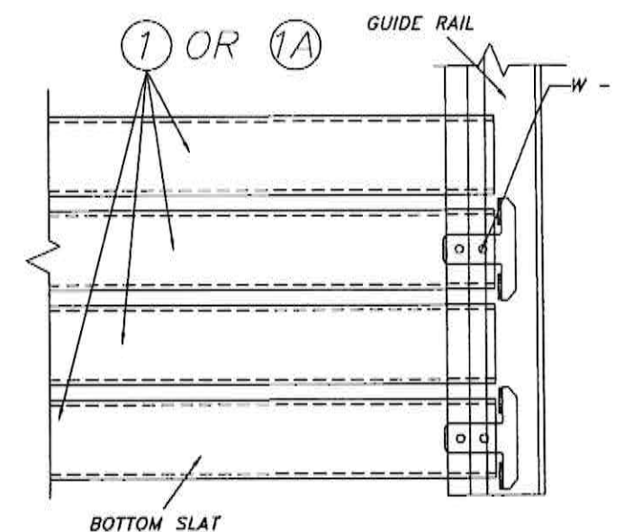
DETAIL 1 (elevation) N.T.S.
