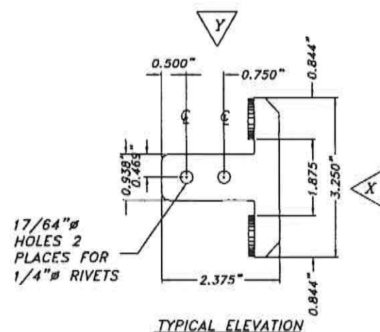
③ TYPICAL WINDLOCK W - 1 DETAIL SCALE : 3/8" = 1"
