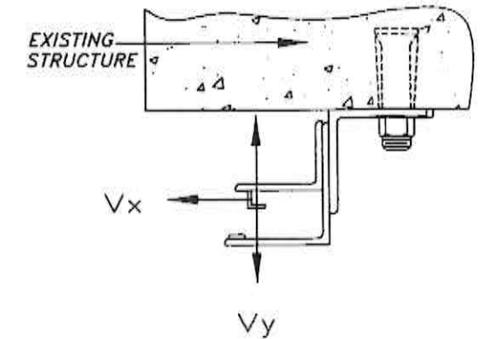
LOAD DIAGRAM
